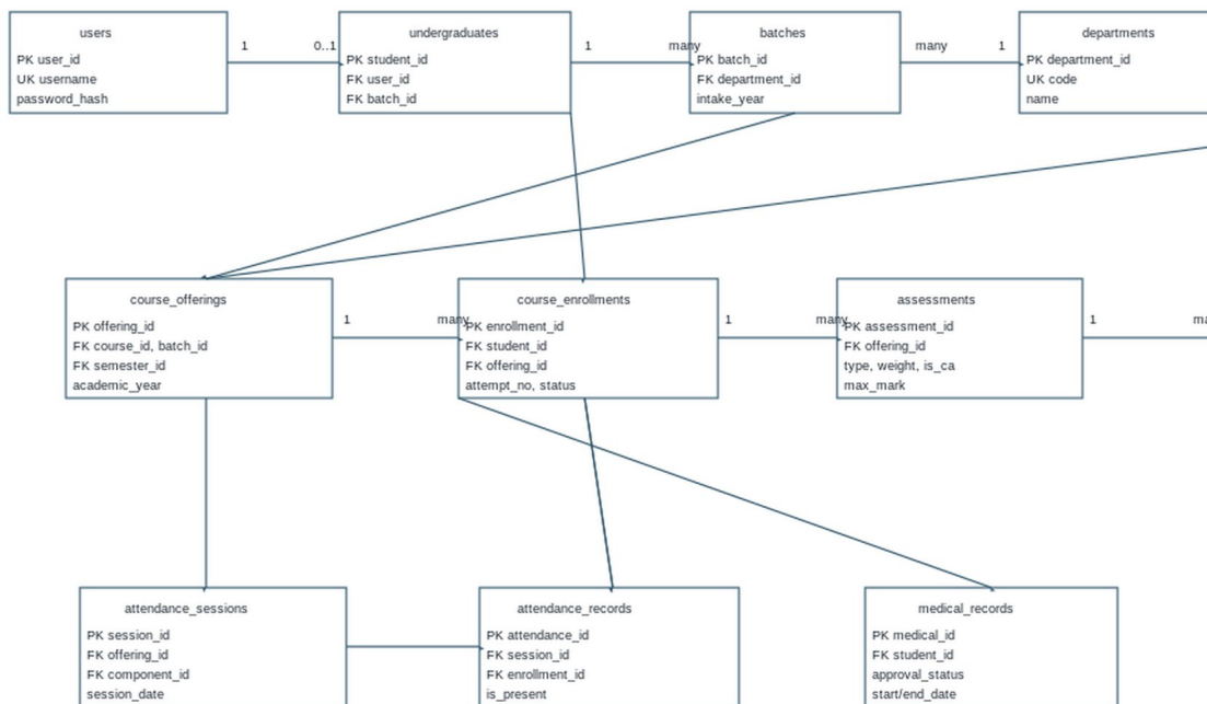
Figure 16. MySQL ER diagram. Lines identify valid FK-to-PK relationships; enrolments, marks and attendance records resolve many-to-many relationships.
