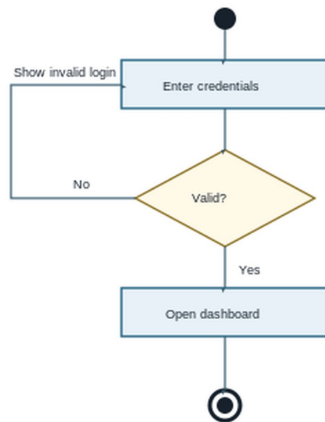
Figure 6. Login activity — alternative invalid-login path returns to credential entry.
